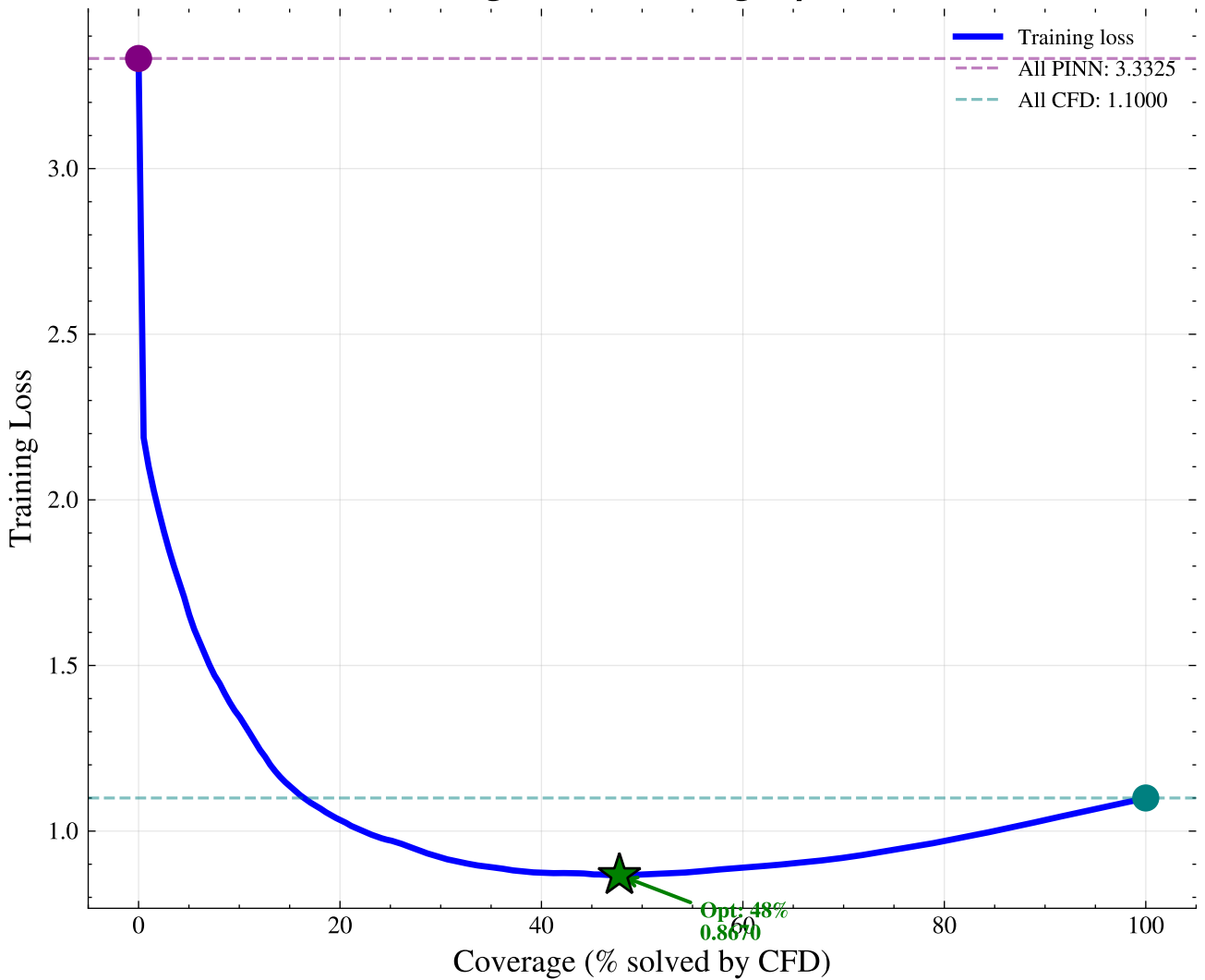
Training Loss vs Coverage ( \beta = 1.1 )
